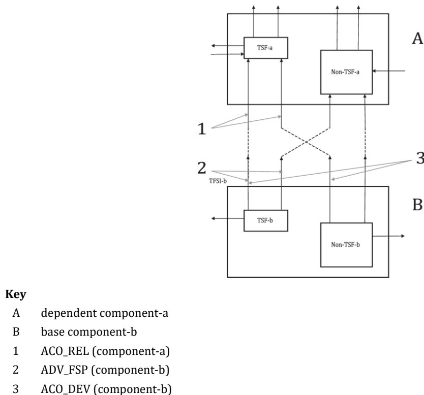
Figure 13 — Relationship between ACO families and interactions between components
