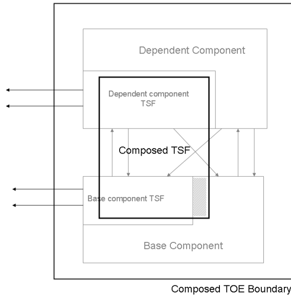
Figure 25 - Composed TOE abstraction
