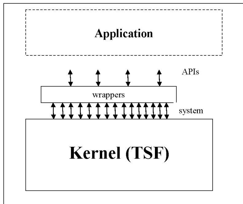
Figure 20 - Wrappers
