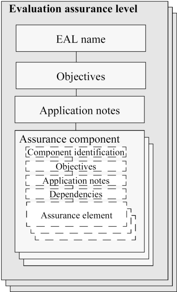
Figure 4 - EAL structure
