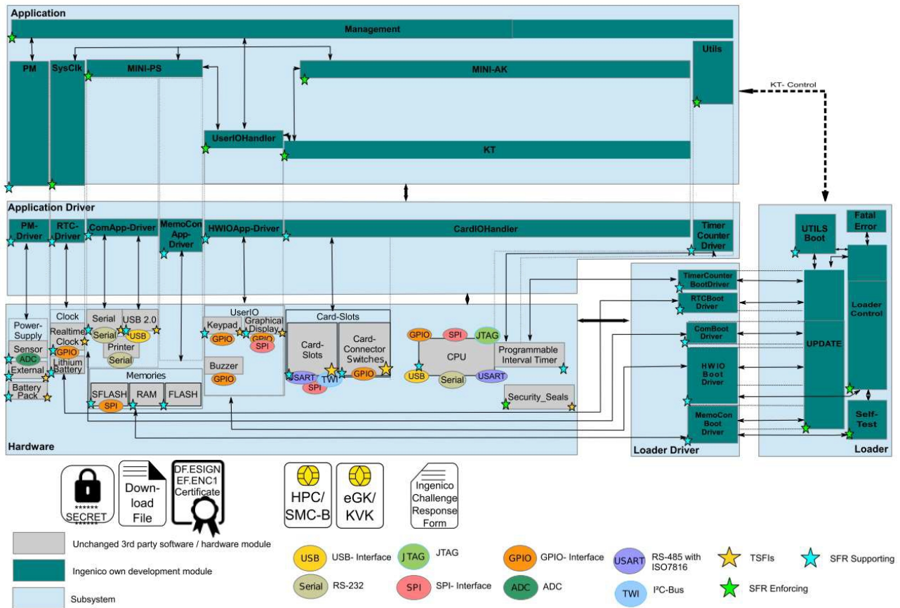
Figure 1: TOE Architecture
