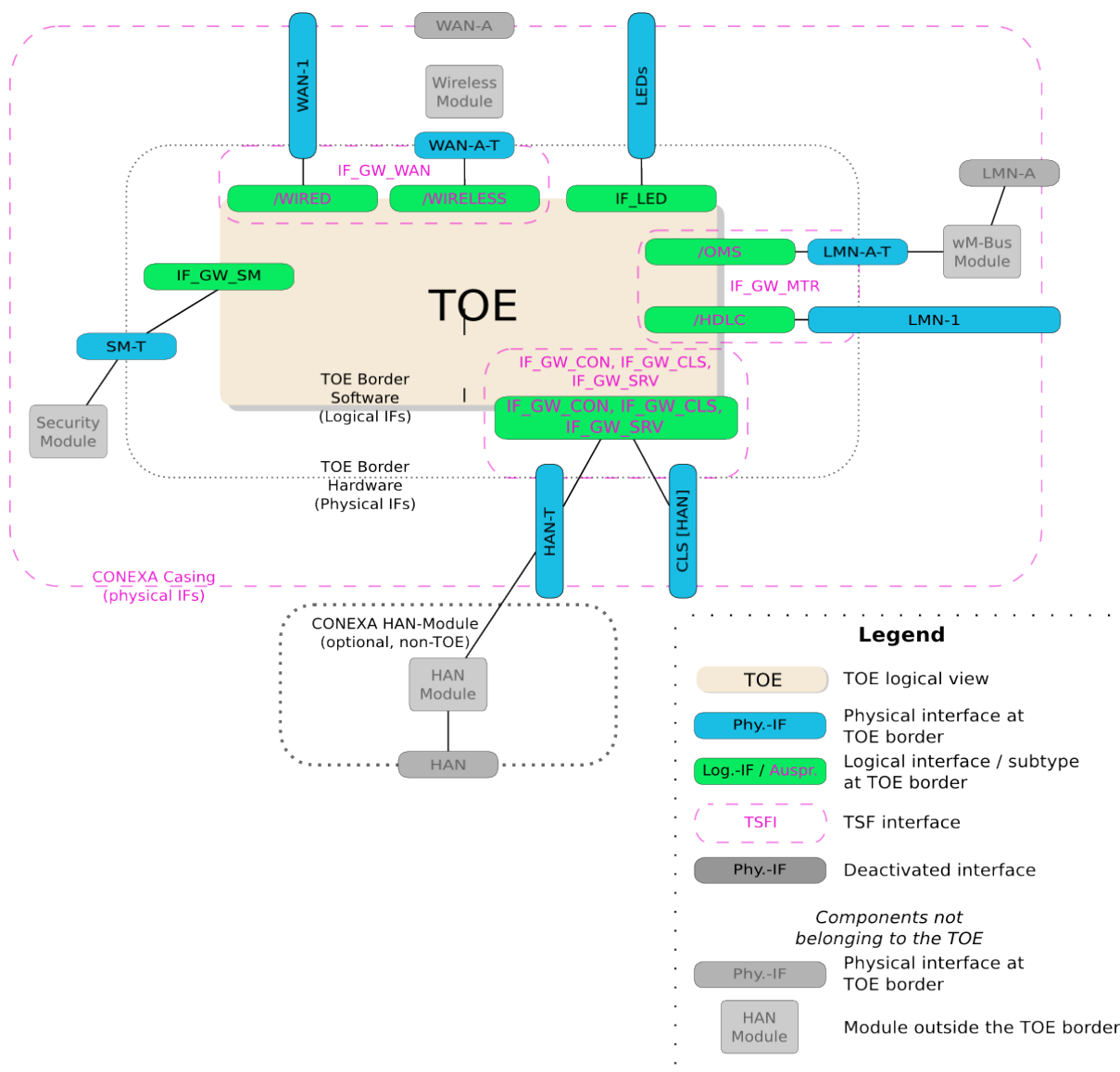
Figure 1.3: Overview of the interfaces of the CONEXA 3.0 SMGW
