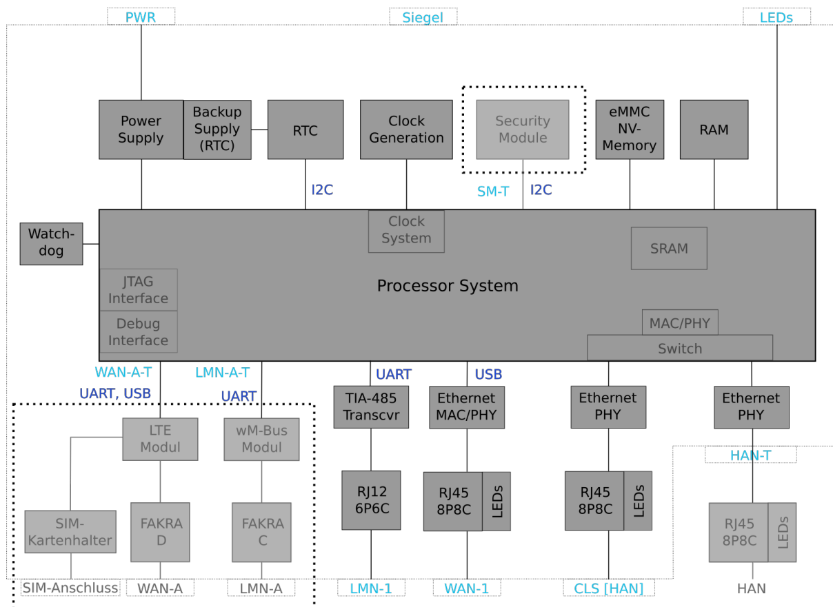
Figure 1.6: The hardware parts of the TOE
