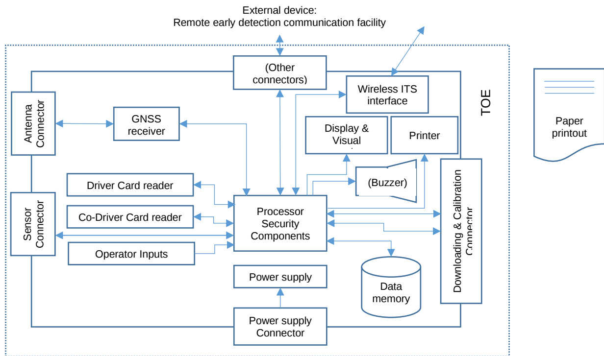
Figure 1 - TOE configuration
