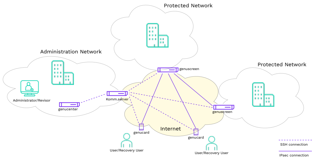
Figure 1: One genucenter managing two genscreens and two genucards (not part of the TOE). The appliances connect to the genucenter through the communication server.
