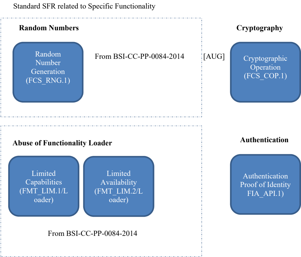
Figure 10 Security Functional Requirements related to Specific Functionality
