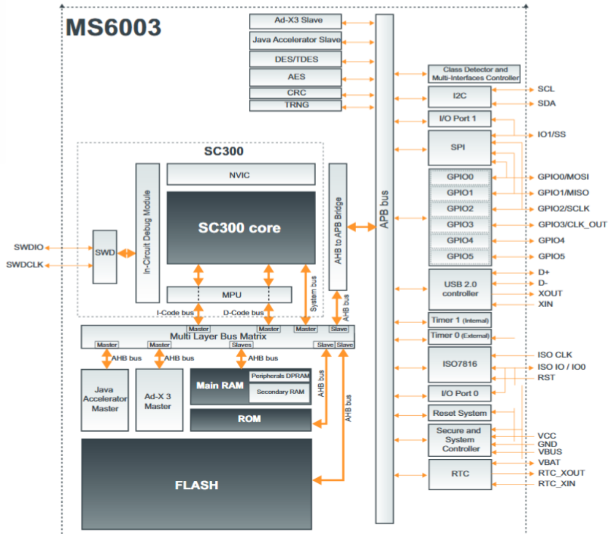
Figure 1 Block Diagram of the MS6003 TOE
