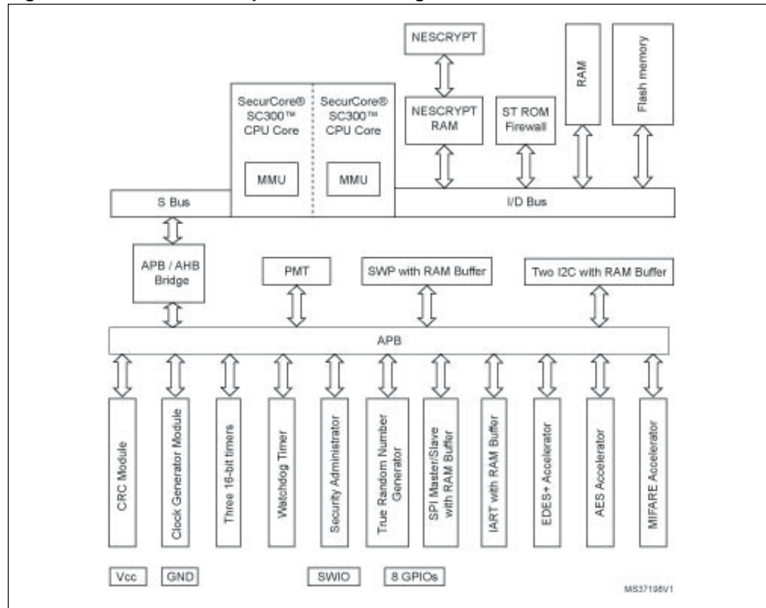
Figure 1. ST33J2M0 C04 platform block diagram
