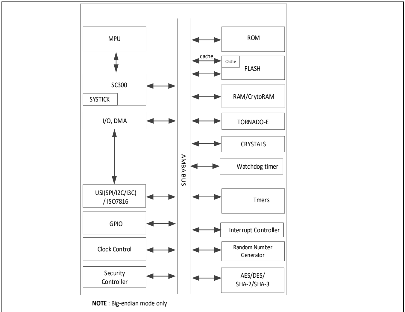
Figure 1 S3SSE2A Block Diagram
