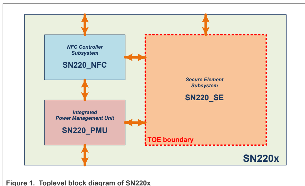
Figure 1. Toplevel block diagram of SN220x
