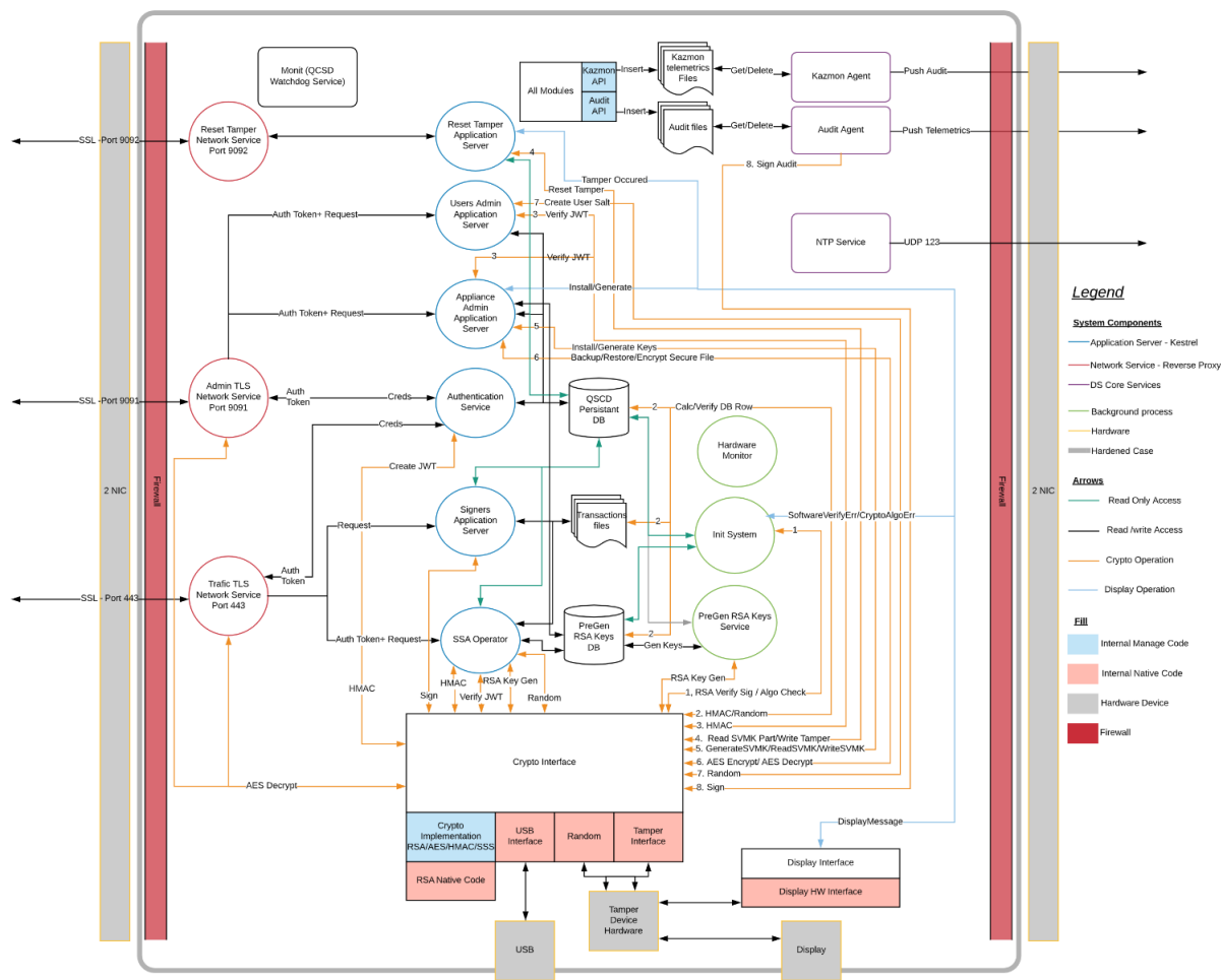
Figure 2 Logical architecture of the TOE.
