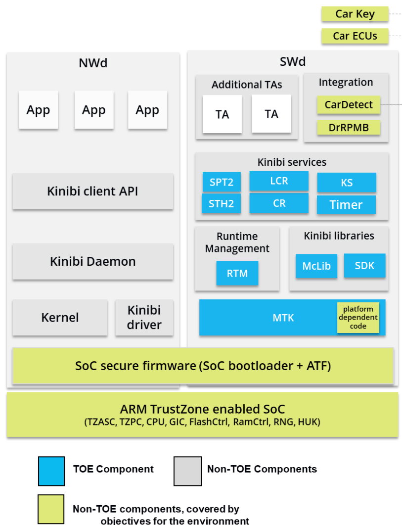
Figure 1: Illustration of Software components
