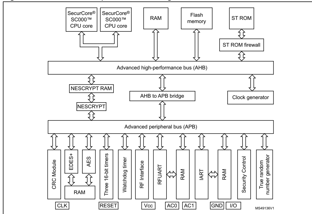
Figure 1. ST31P450 A05 platform block diagram
