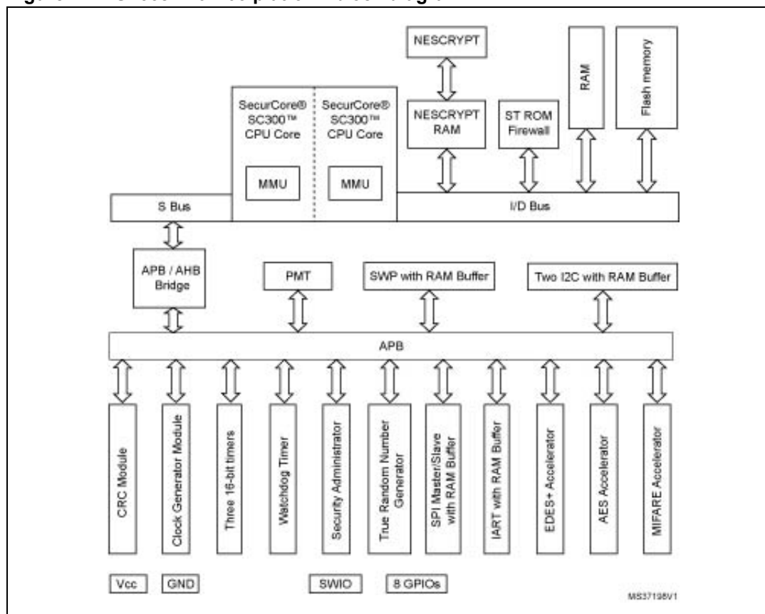
Figure 1. ST33J2M0 D03 platform block diagram
