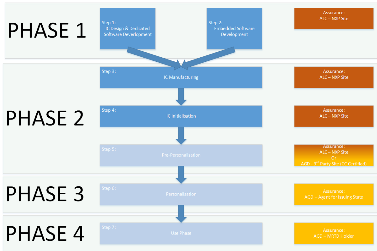
Fig 2. TOE LifeCycle
