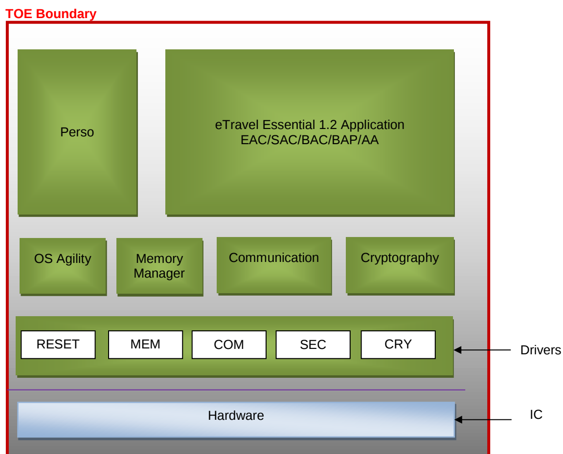
Figure 1: TOE Boundary
