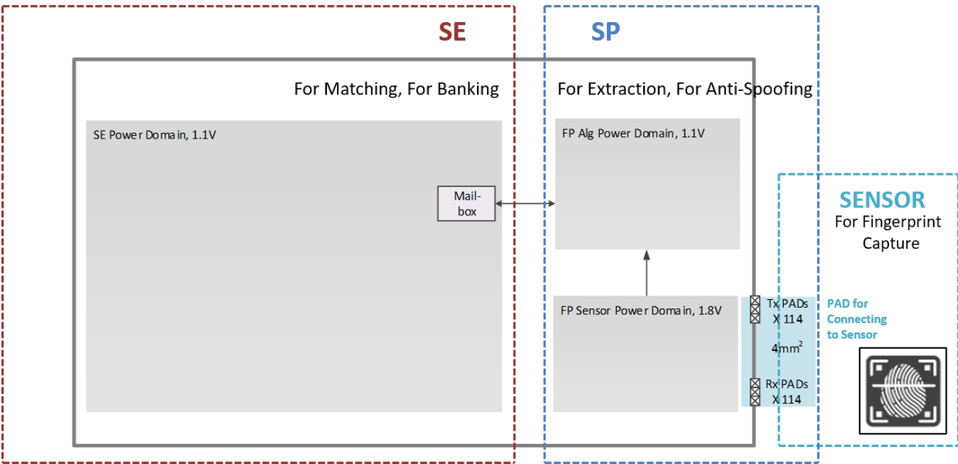
Figure 1-2 S3B512C/SC3512C Architecture
