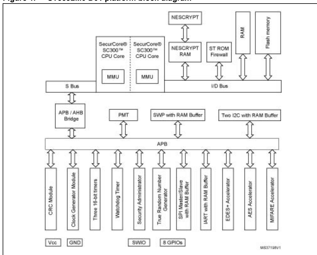
Figure 1. ST33J2M0 D01 platform block diagram
