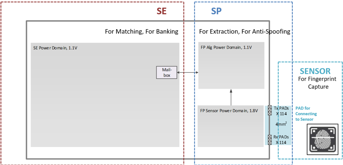
Figure 1-2 S3B512C/SC3512C Architecture
