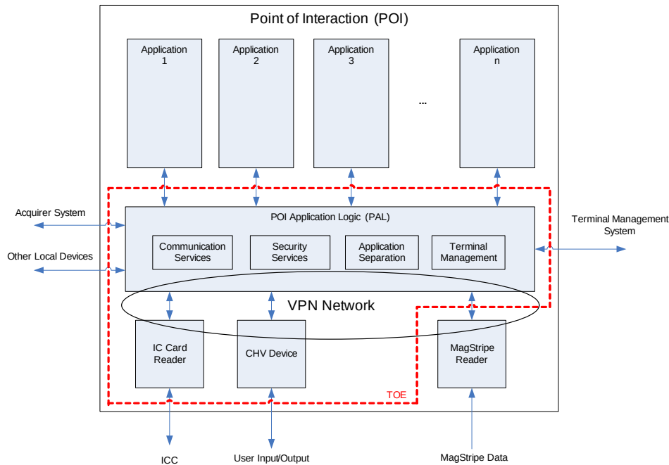
Figure 1 Configuration POI-CHIP-ONLY
