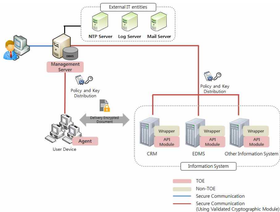
[Figure 2] Operational environment of “Information system encryption” type
