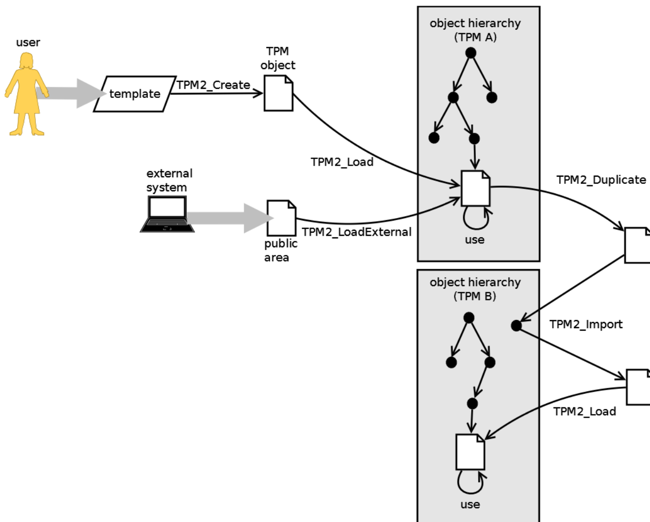
Figure 4: Object Export/Import Scenarios (informative)
