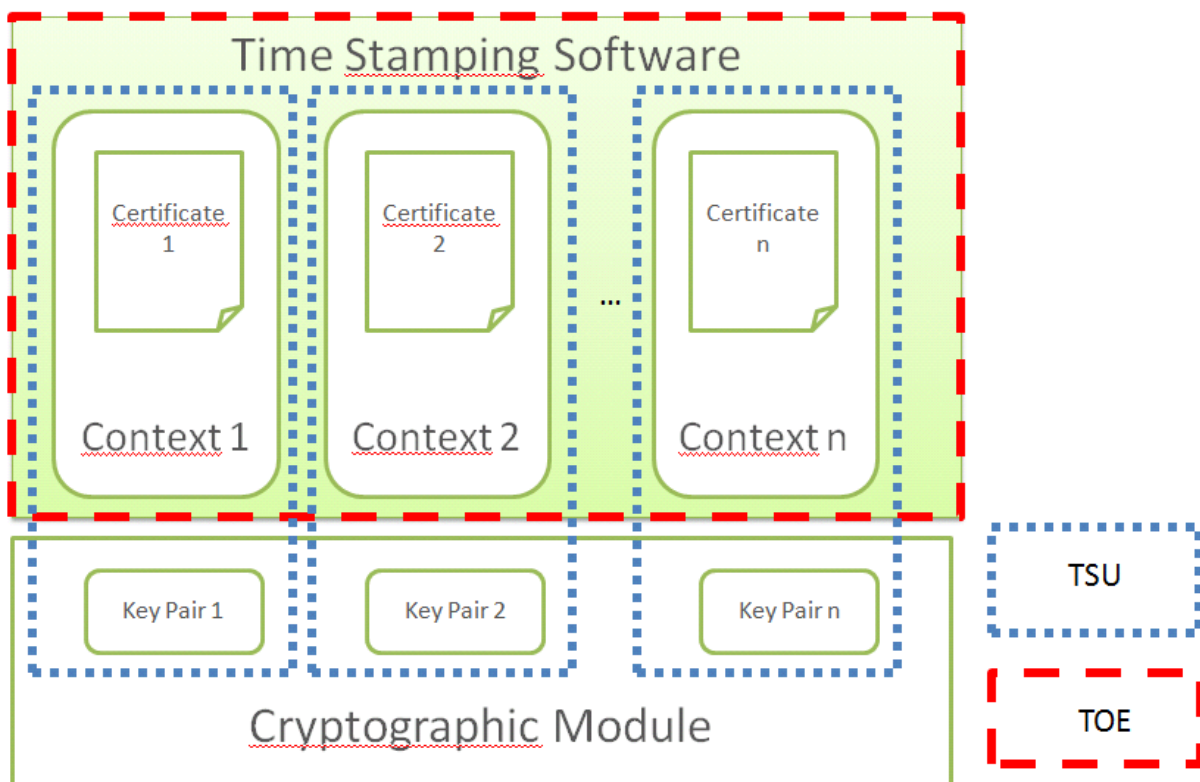
Figure 4. Time-stamping Unit
