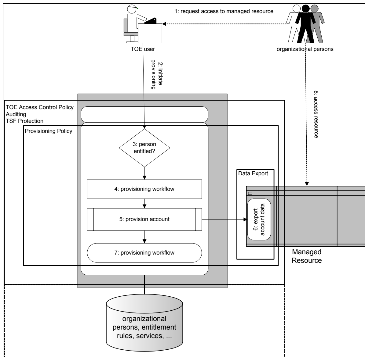
Figure 2: A provisioning workflow and the scope of the TSP
